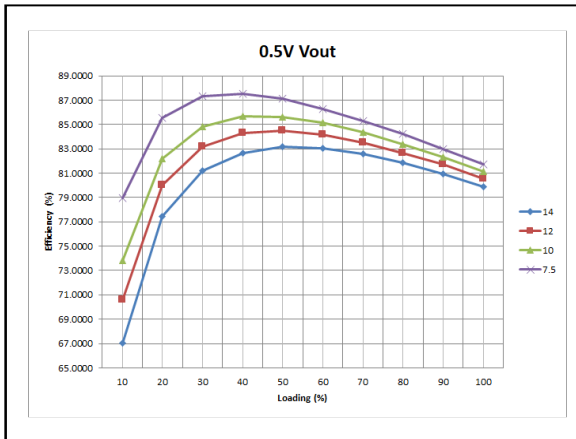
Figure 1: LGA110D-00DADJJB Efficiency Curves at different V_{IN} @ 25°C Loading: I_O = 10% increment to 110A, V_O = 0.5V Frequency=533KHz
