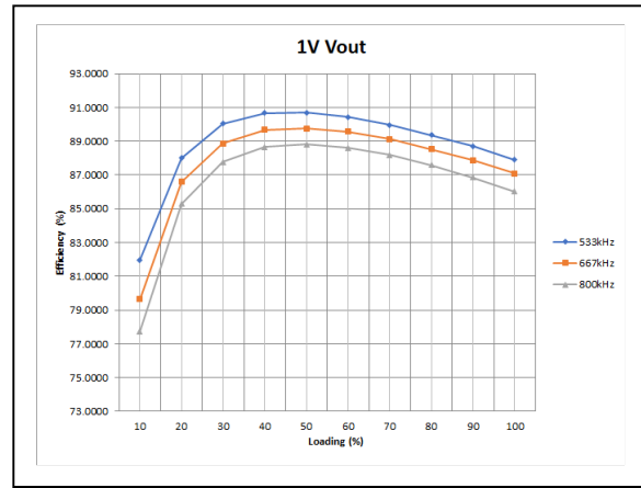
Figure 8: LGA110D-01DADJJB Efficiency Curves at different switching frequency @ 25°C, Vin = 12V Loading: I o = 10% increment to 110A
