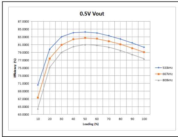
Figure 7: LGA110D-01DADJJB Efficiency Curves at different switching frequency @ 25°C, Vin = 12V Loading: I o = 10% increment to 110A
