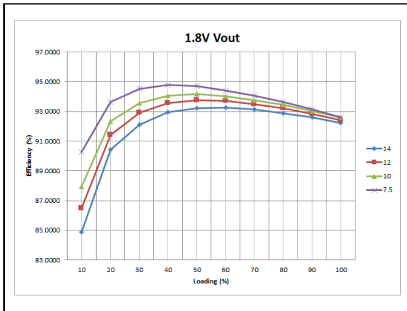
Figure 3: LGA110D-01DADJJB Efficiency Curves at different V_{IN} @ 25°C Loading: I_O = 10% increment to 100A, V_O = 1.8V Frequency=533KHz
