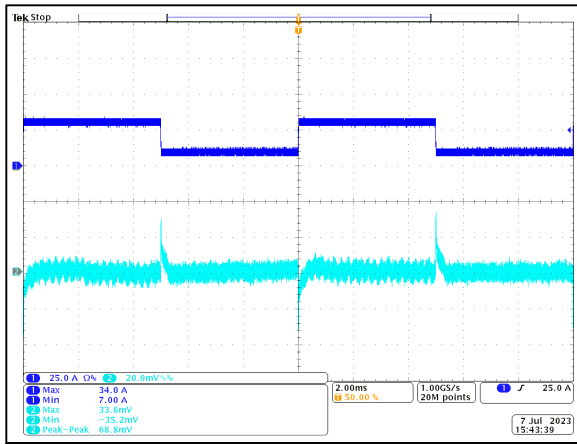
Figure 34: LGA110D-01DADJJB Transient Response - Vo Deviation 25% to 75% to 25% load change, 1A/ \mu S slew rate, Vin = 12Vdc Vo = 3.3V Ch 1: Io Ch 2: Vo F SW =533kHz
