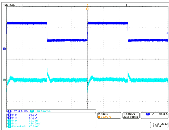
Figure 40: LGA110D-01DADJJ Transient Response - Vo Deviation 25% to 75% to 25% load change, 1A/ \mu S slew rate, Vin = 12Vdc Vo = 3.3V Ch 1: I_O Ch 2: V_O F_{SW} =533kHz
