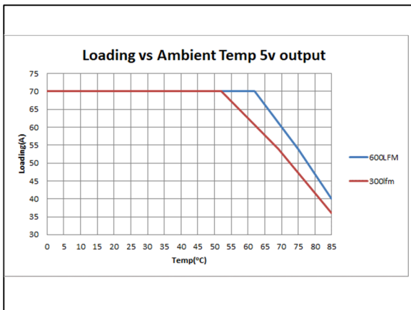
Figure 17: LGA110D-01DADJJB Thermal Derating Curves (Two modules with Longitudinal airflow) Vin = 14V Load: I O = 36 to 70A, V O = 5.0V F SW = 533kHz
