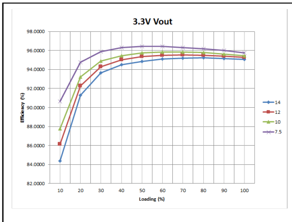
Figure 5: LGA110D-01DADJJB Efficiency Curves at different V_{IN} @ 25°C Loading: I_O = 10% increment to 80A, V_O = 3.3V Frequency=533KHz
