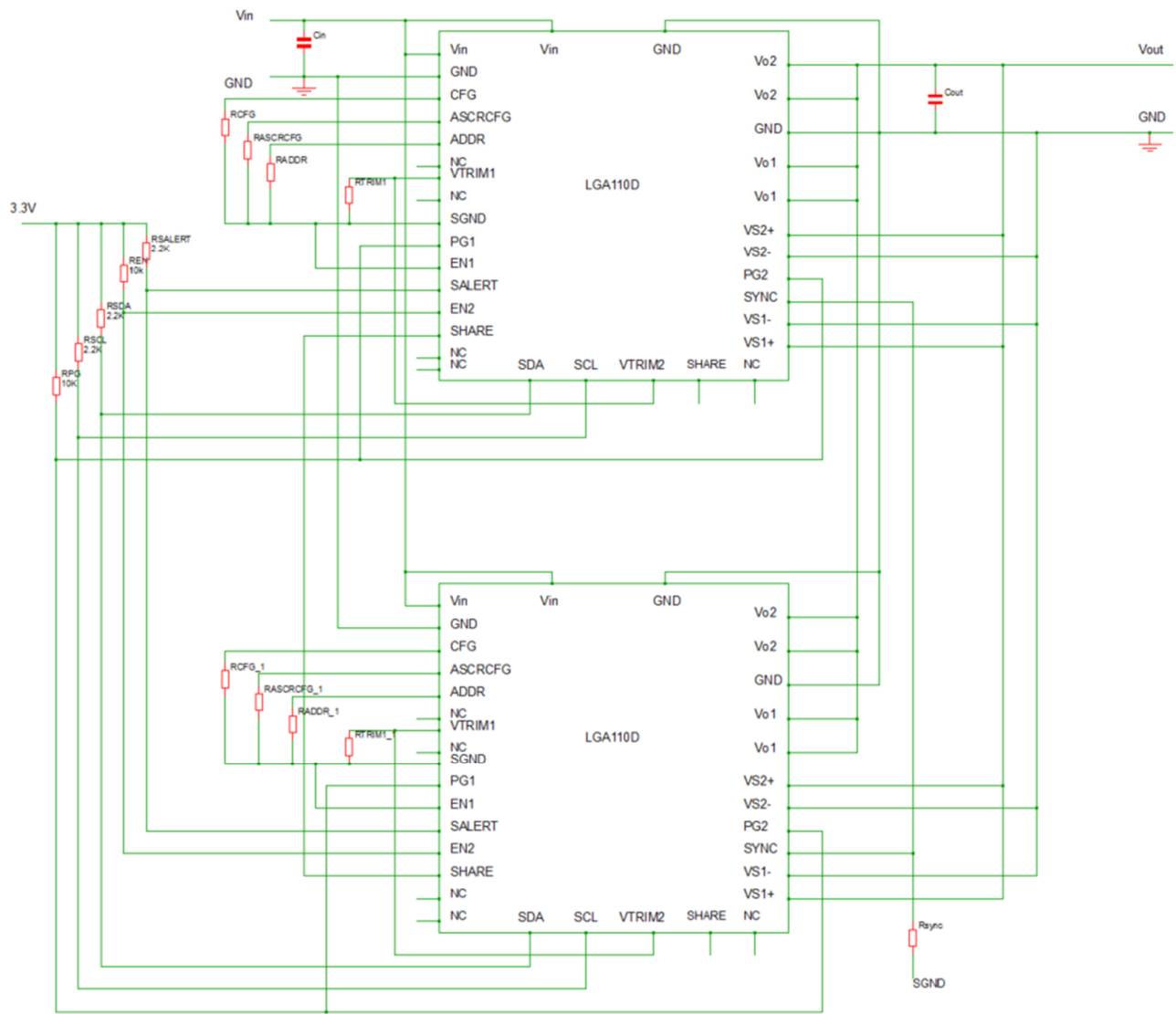
Figure 59: Two modules one output
