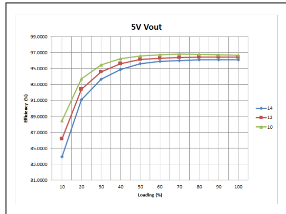
Figure 6: LGA110D-00DADJJB Efficiency Curves at different V_{IN} @ 25°C Loading: I_O = 10% increment to 70A, V_O = 5V Frequency=533KHz
