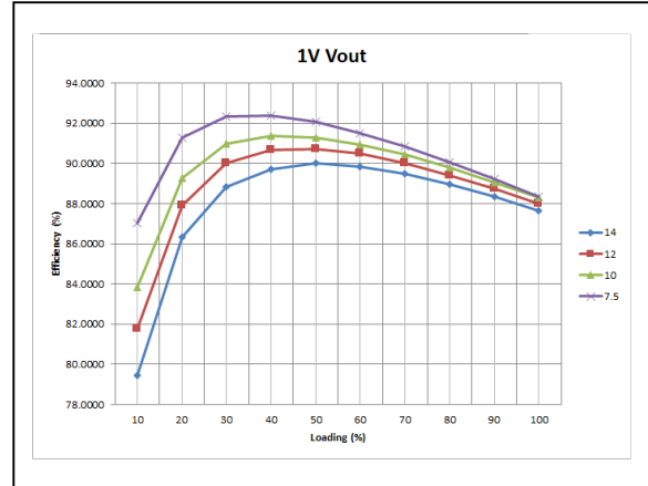
Figure 2: LGA110D-01DADJJB Efficiency Curves at different V_{IN} @ 25°C Loading: I_O = 10% increment to 110A, V_O = 1V Frequency=533KHz
