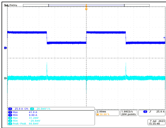
Figure 32: LGA110D-01DADJJB Transient Response - Vo Deviation 25% to 75% to 25% load change, 1A/ \mu S slew rate, Vin = 12Vdc Vo = 1.8V Ch 1: Io Ch 2: Vo F SW =533kHz
