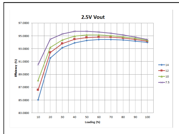
Figure 4: LGA110D-01DADJJB Efficiency Curves at different V_{IN} @ 25°C Loading: I_O = 10% increment to 90A, V_O = 2.5V Frequency=533KHz
