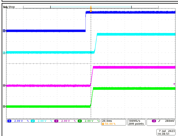
Figure 28: LGA110D-01DADJJB Start Up - V_o = 3.3V Full Load Ch 1: Enable Ch 2: V_{O1} Ch 3: V_{O2} Ch 4: V_{O3}
