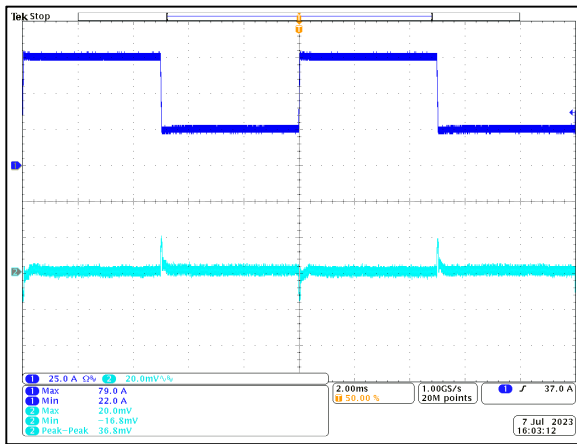
Figure 38: LGA110D-01DADJJ Transient Response - Vo Deviation 25% to 75% to 25% load change, 1A/ \mu S slew rate, Vin = 12Vdc Vo = 1.8V Ch 1: I_O Ch 2: V_O F_{SW} =533kHz
