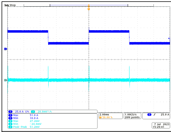
Figure 30: LGA110D-01DADJJB Transient Response - Vo Deviation 25% to 75% to 25% load change, 1A/ \mu S slew rate, Vin = 12Vdc Vo = 0.5V Ch 1: Io Ch 2: Vo F SW =533kHz
