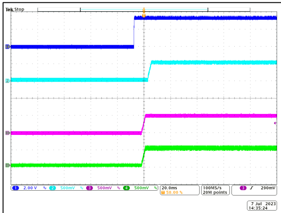
Figure 24: LGA110D-01DADJJB Start Up - V_o = 0.5V Full Load Ch 1: Enable Ch 2: V_{O1} Ch 3: V_{O2} Ch 4: V_{O3}
