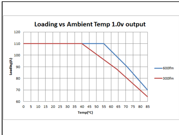
Figure 13: LGA110D-01DADJJB Thermal Derating Curves (Two modules with longitudinal airflow) Vin = 14V Load: I O = 64 to 110A, V O = 1.0V F SW = 533kHz
