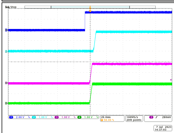
Figure 26: LGA110D-01DADJJB Start Up - V_o = 1.8V Full Load Ch 1: Enable Ch 2: V_{O1} Ch 3: V_{O2} Ch 4: V_{O3}
