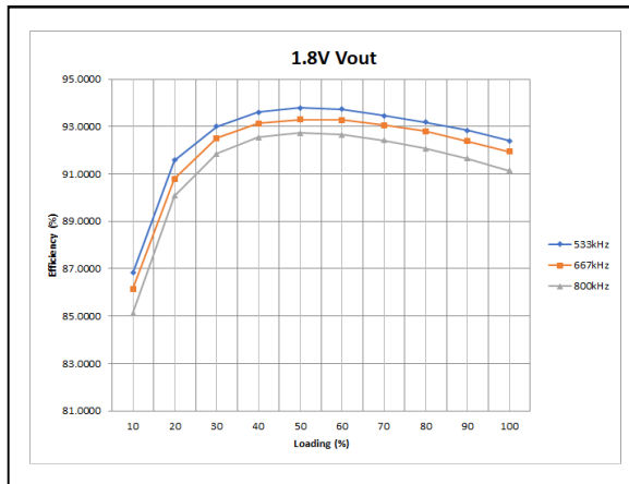
Figure 9: LGA110D-01DADJJB Efficiency Curves at different switching frequency @ 25°C, Vin = 12V Loading: I o = 10% increment to 100A
