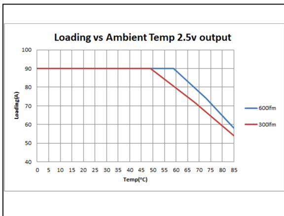
Figure 15: LGA110D-01DADJJB Thermal Derating Curves (Two modules with Longitudinal airflow) Vin = 14V Load: I O = 54 to 90A, V O = 2.5V F SW = 533kHz
