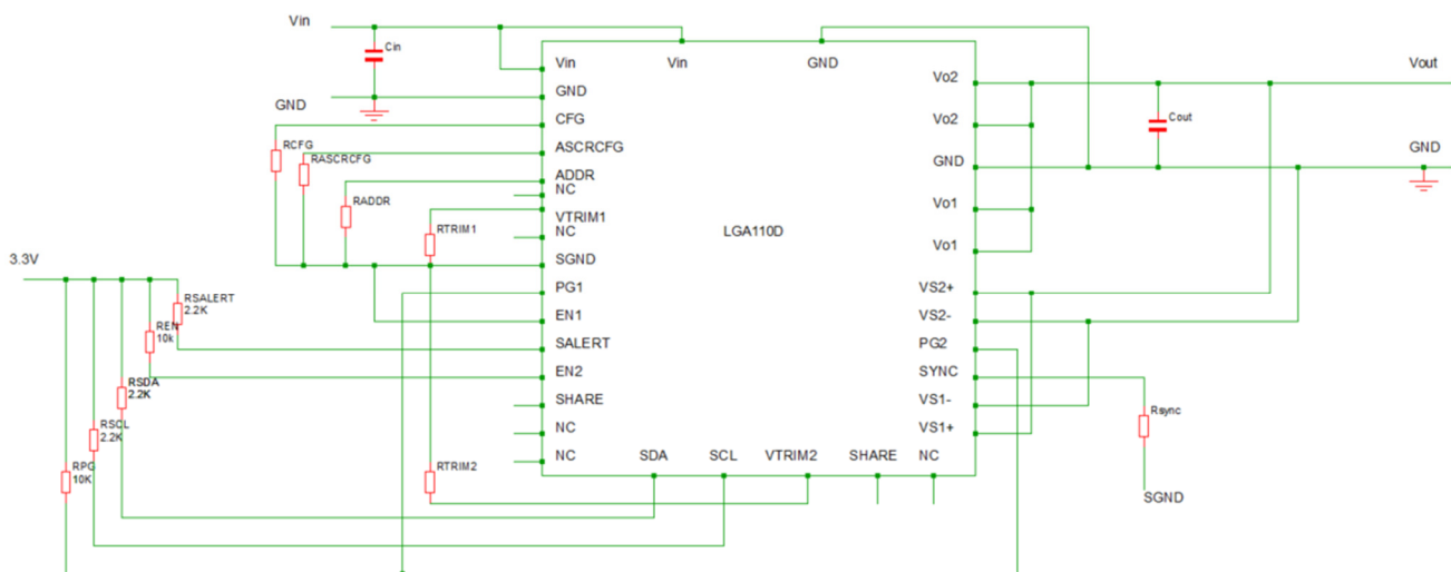
Figure 57: One module one output
