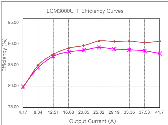
Figure 53: LCM3000U-T Efficiency Curve @ 25°C Loading: Io_main = 10%Io_max increment to 41.7A, Isb = 0A ◆ 115Vac ◆ 90Vac
