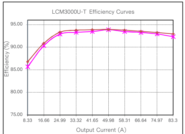
Figure 54: LCM3000U-T Efficiency Curve @ 25°C Loading: Io_main = 10%Io_max increment to 83.3A, Isb = 0A ◆ 264Vac ◆ 230Vac
