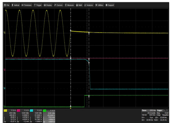
Figure 6: LCM3000L-T Hold-up Time Vin = 264Vac Load: Io = 250A (12V), Isb = 2A Ch 1: Vin Ch 2: Vsb Ch 3: Vo Ch 4: G_DCOK_C
