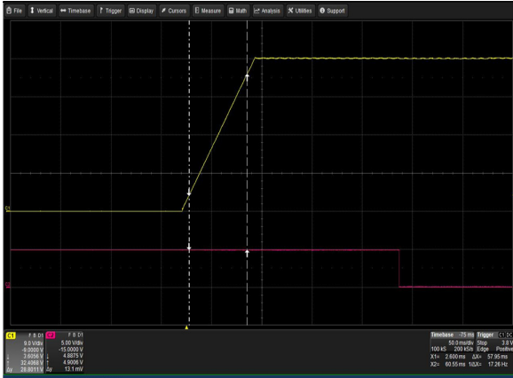
Figure 49: LCM3000U-T Output Voltage Startup Vin = 264Vac Load: Io = 83.3A (36V), Isb = 2A Ch 1: Vo Ch 2: G_DCOK_C
