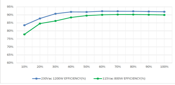
Figure 7. Efficiency Curves for LCC1200-48U with 42 V Output
