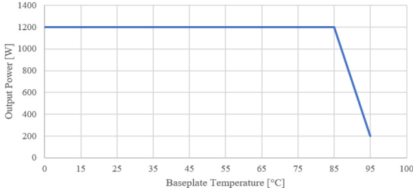
Figure 2. Output Power vs. Baseplate Temperature (180 VAC to 264 VAC)
