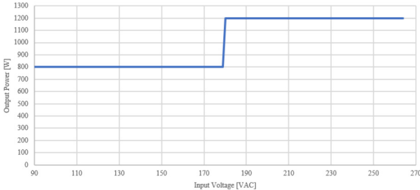
Figure 3. Output Power vs. Input Voltage
