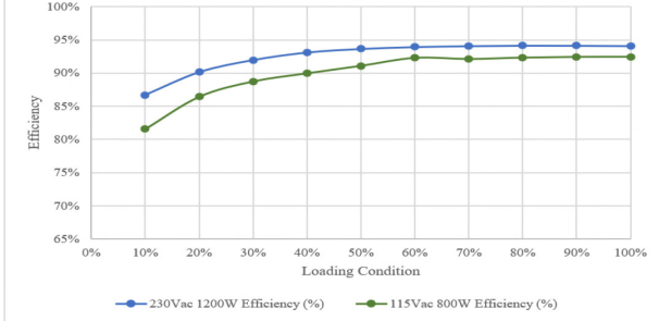
Figure 5. Efficiency Curves for LCC1200-28U with 28 V Output
