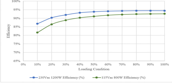
Figure 6. Efficiency Curves for LCC1200-28U with 30 V Output
