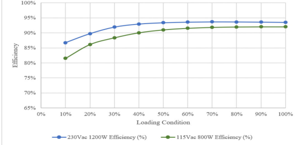
Figure 4. Efficiency Curves for LCC1200-28U with 24 V Output
