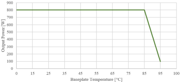
Figure 1. Output Power vs. Baseplate Temperature (90 VAC to 179 VAC)
